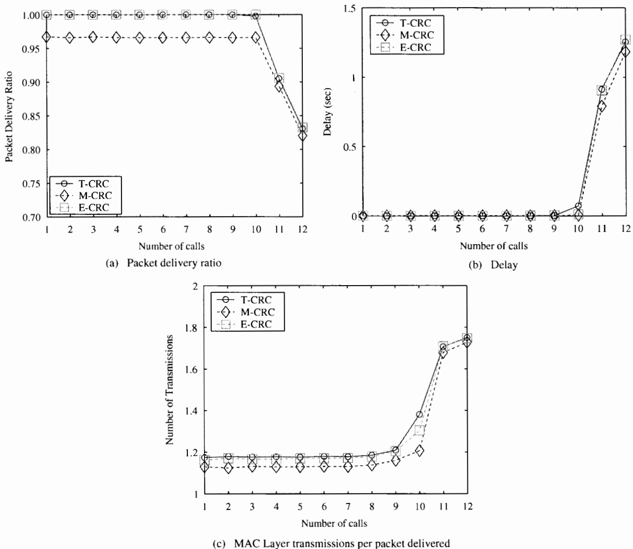
Fig. 7. G.723.1 encoder results.
