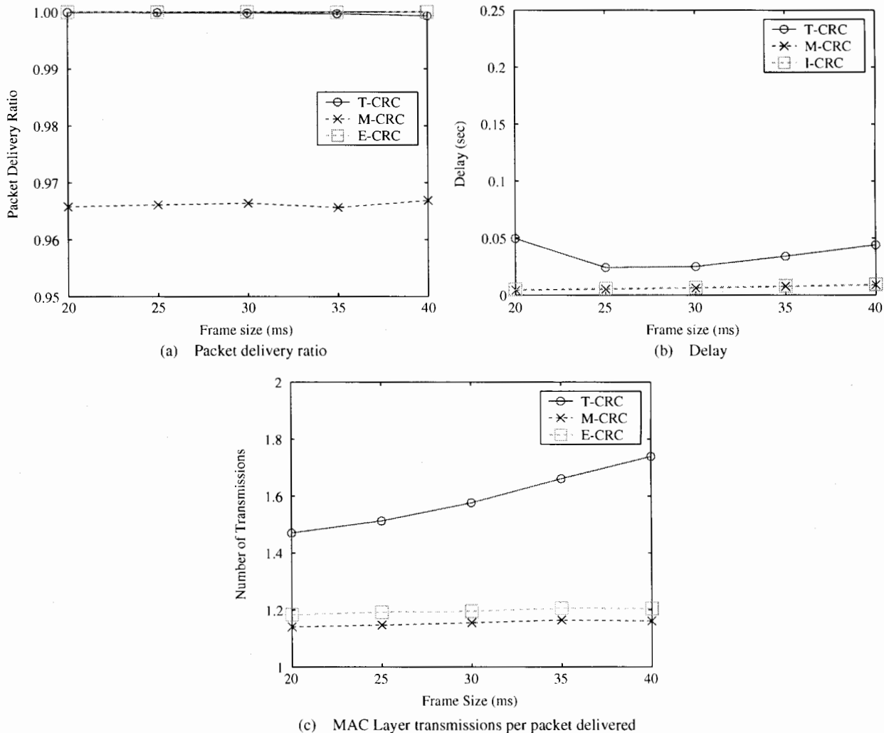
Fig. 8. Voice frame size results.
