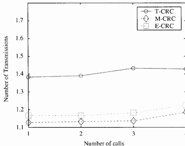
(c) MAC Layer transmissions per packet delivered
