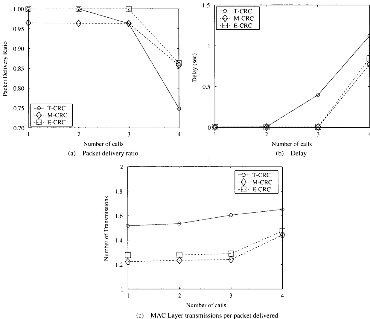
Fig. 9. Interference limited (IL) error model results.
