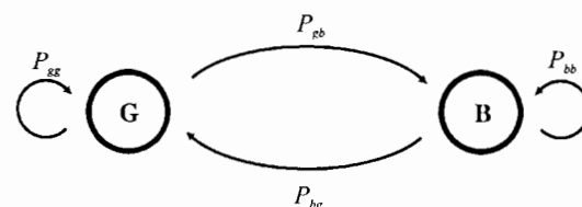
Fig. 2. Gilbert error model state diagram.
