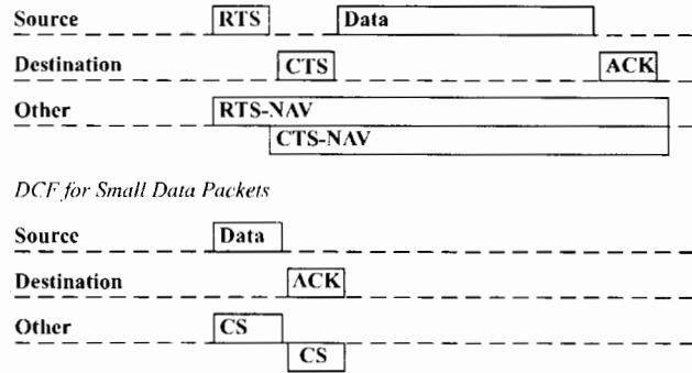
Fig. 1. IEEE 802.11 distributed coordination function.
